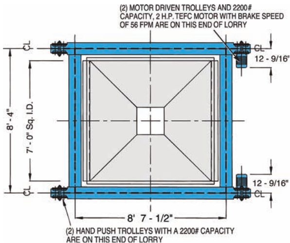
WEIGH LORRY PLAN VIEW
